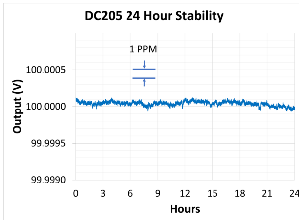
DC205 Stability
